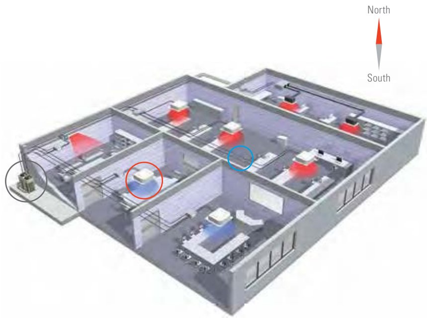
Refrigerant piping
